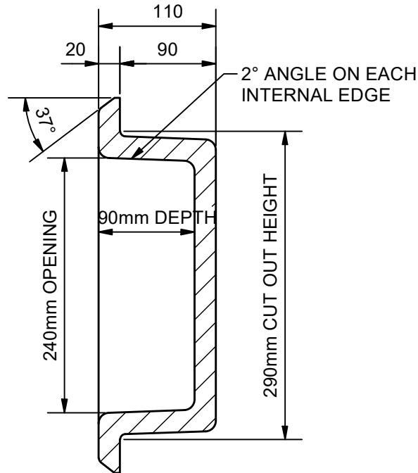
SECTION VIEW A-A ( SCALE 1:5 )
